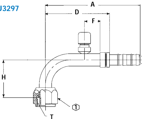
90° Female O-ring (Short Pilot) with Switch Port (M10 X 1.25)
