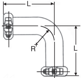
Basic part number: NH1627 NH1677 Allowable misalignment: \pm 2' per end
